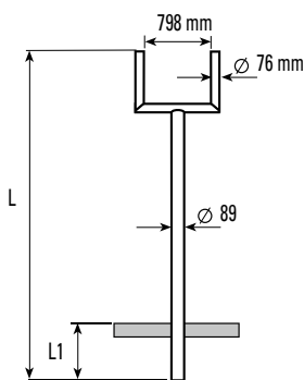
RM89/76/2/3600 C (L = 3600, L1 = 600)
