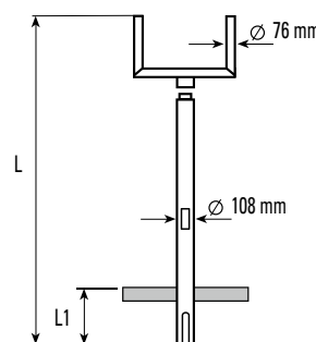
GE 108/3600 (L = 3600, L1 = 800)
