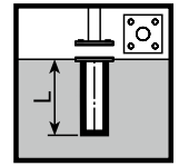
FL4A FL4B Flanschbefestigung Flasque de fixation Ø 150 | Ø 200 L = 300 | L = 300 L = 400 | L = 400 L = 500 | L = 500
